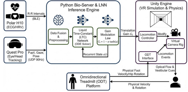
Figure 1: System architecture. High-frequency ocular telemetry and irregular cardiac intervals are fused via the Liquid Neural Network to modulate translation gain.
